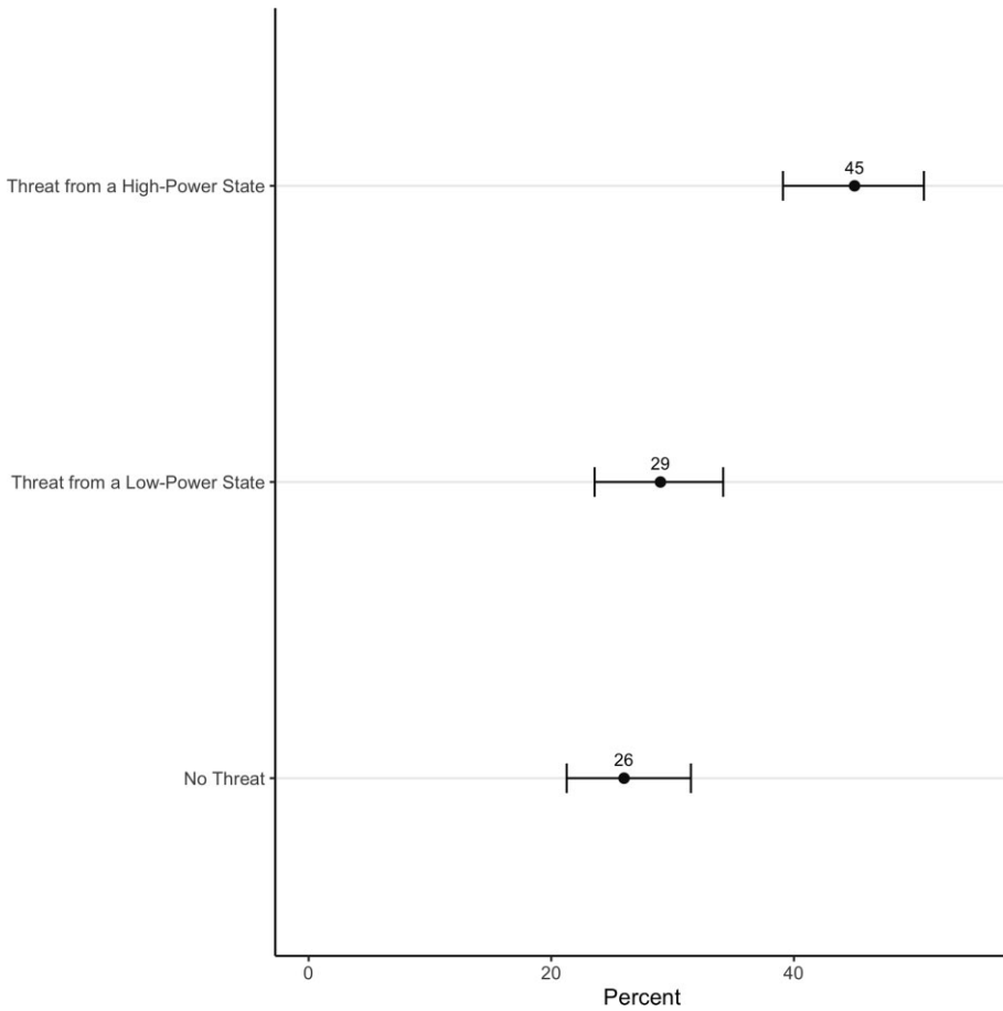
Figure 1. Support for proliferation under different types of external security environment. Note: The points are estimates and the horizontal bars are 95 percent confidence intervals.
