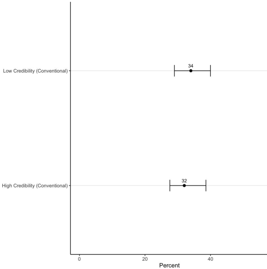
Figure 3. Support for proliferation under different levels of credibility of US conventional security guarantees. Note: The points are estimates and the horizontal bars are 95 percent confidence intervals.
